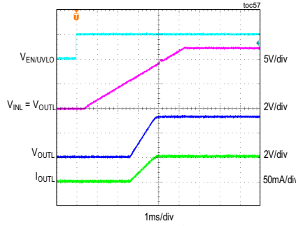
MAX17671F, 3.3V LINEAR REGULATOR START-UP FROM ENUVLO FIGURE 6 CIRCUIT
