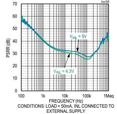
MAX17671F, 3.3V OUTPUT LINEAR REGULATOR, POWER SUPPLY REJECTION RATIO vs. FREQUENCY
