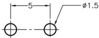
MOUNTING HOLES
