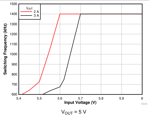
Figure 7-10. Frequency Foldback
