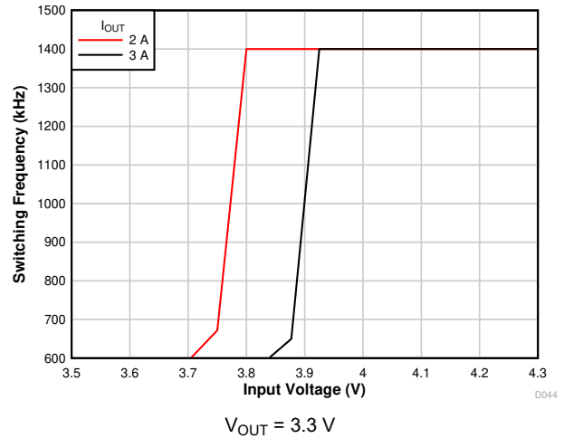
Figure 7-8. Frequency Foldback
