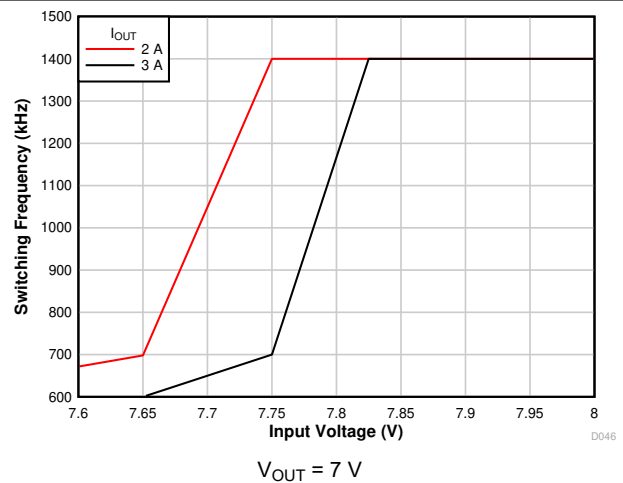
Figure 7-12. Frequency Foldback
