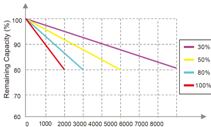
Cycle Life Curves:
