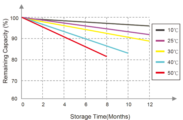
Self-Discharge Curves:
