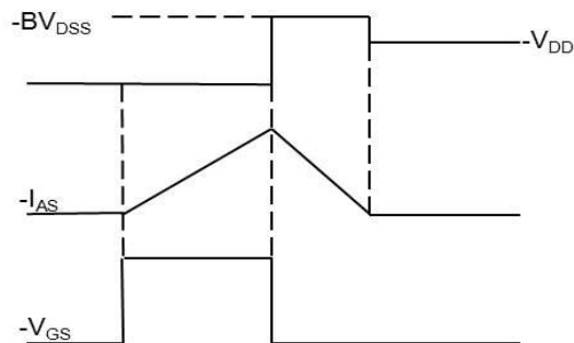
Figure 11. EAS Waveform
