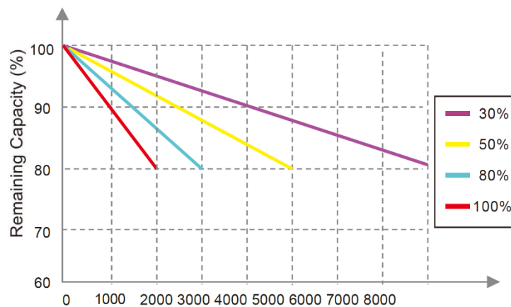
DOD Cycle Life Curves 1C:
