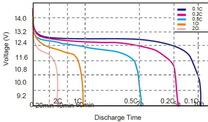
Discharge Rate Curves +25°C:
