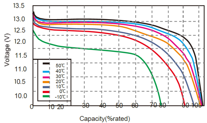
Temperature Discharge Curves 0.5C:
