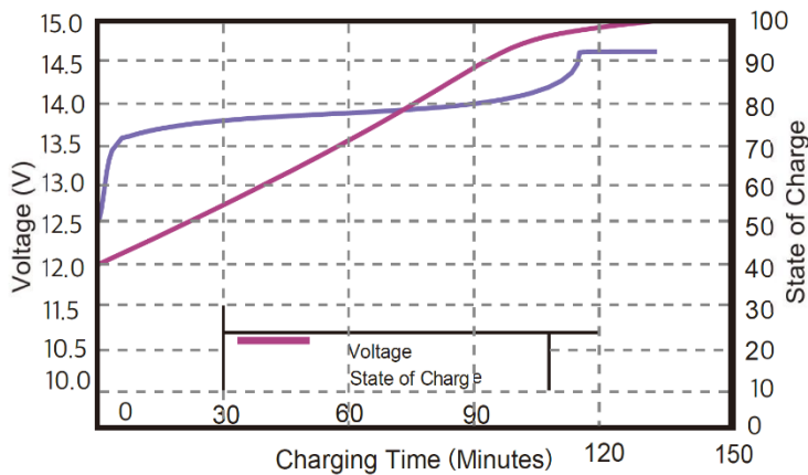
State of Charge Curves 0.5C +25°C:
