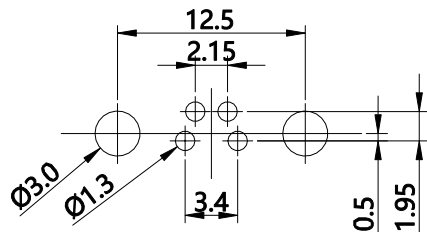
PCB layout PCB thickness: 1.6mm
