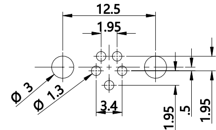
PCB layout( thickness: 1.6mm)
