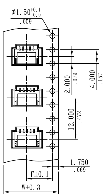
2~13 Circuits
