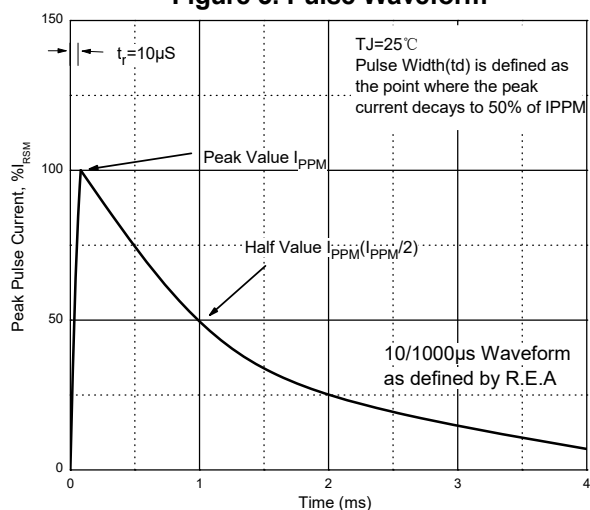
Figure 3. Pulse Waveform
