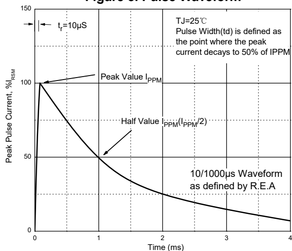
Figure 3. Pulse Waveform
