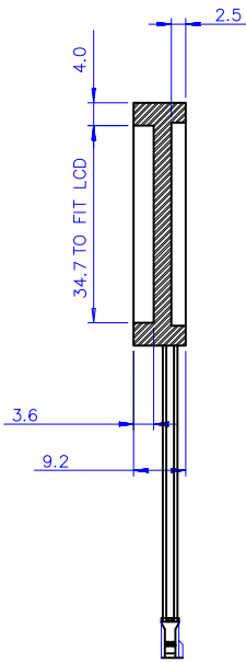
SECTION B-B
