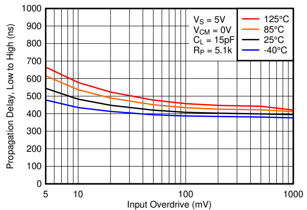
Figure 2-26. Low to High Propagation Delay vs. Input Overdrive Voltage, 5V
