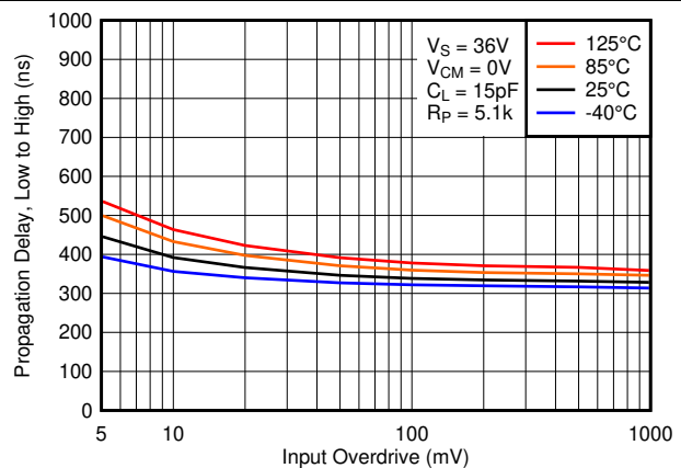
Figure 2-30. Low to High Propagation Delay vs. Input Overdrive Voltage, 36V
