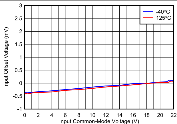
Figure 5-3. Offset vs. Common-Mode, 24V
