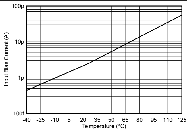
Figure 5-5. Bias Current vs. Temperature, 24V
