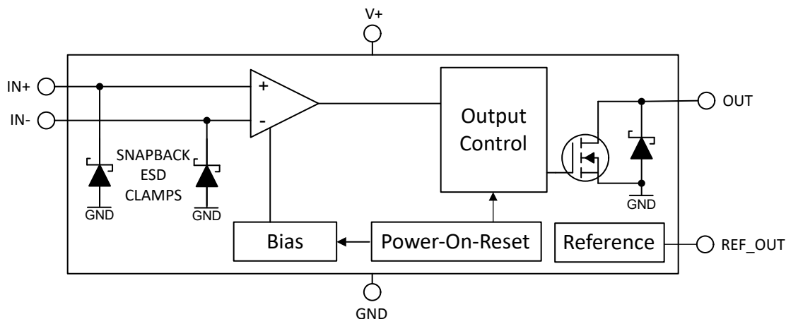
Figure 6-1. Block Diagram
