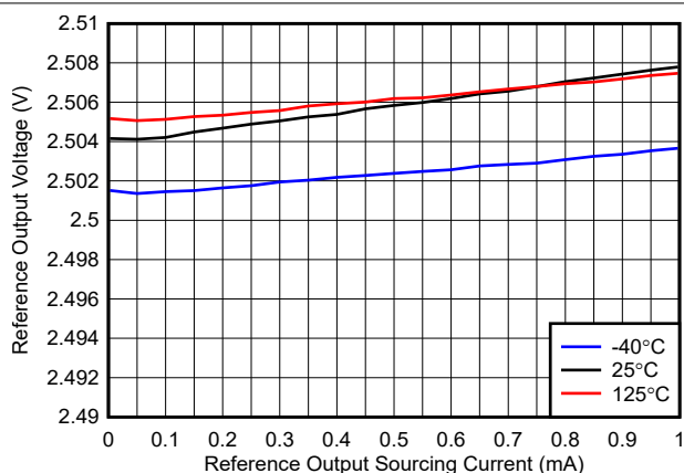
Figure 5-12. Reference Voltage vs. Reference Output Sourcing Current
