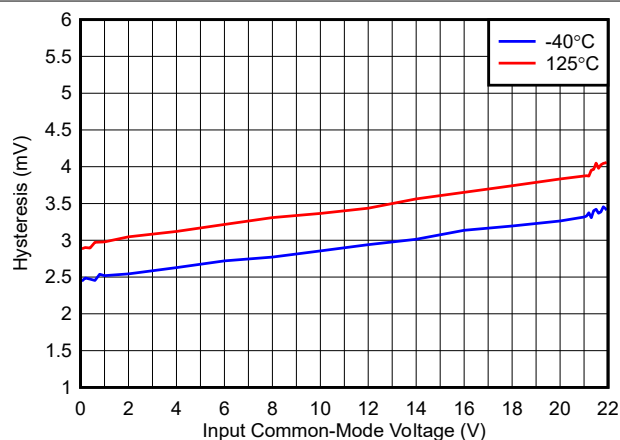
Figure 5-4. Hysteresis vs. Common-Mode, 24V
