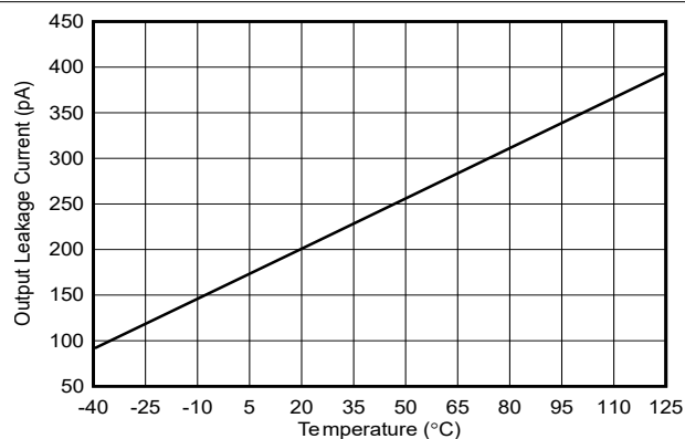
Figure 5-6. Output Leakage Current vs. Temperature
